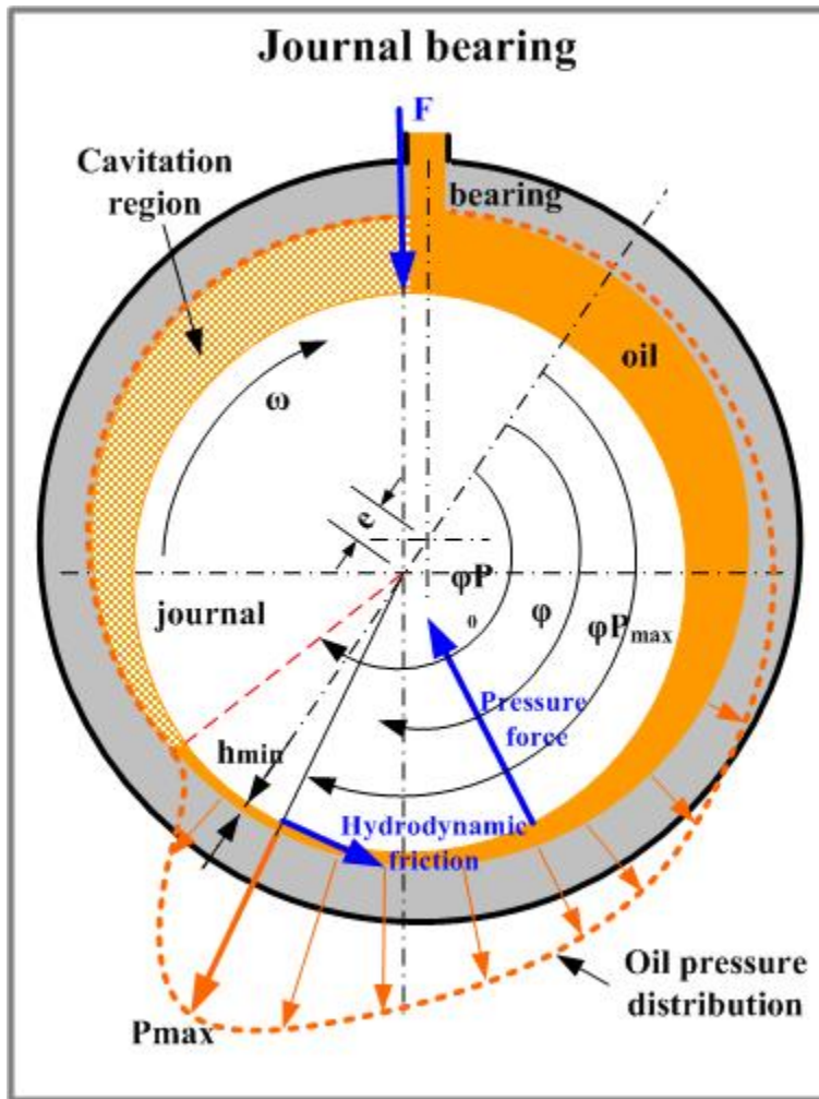
Fig.2 Journal bearing
